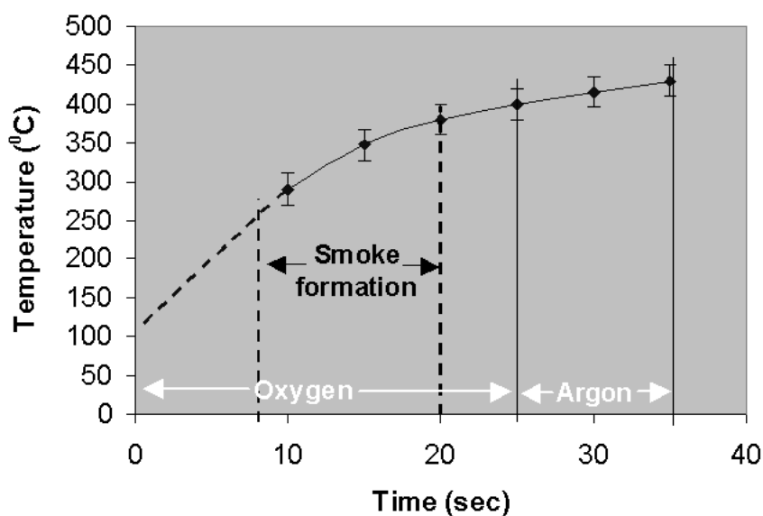
Figure 2. Temperature variation of the inner cup-platform in the ashing step of the atomization cycle.
