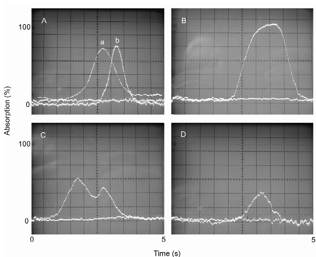
Figure 3. Absorption-time profiles of lead resulting from atomization of aqueous standards and various biological solid samples employing the direct »tape sandwich« introduction technique; A – \text{PbCl}_2 (a), \text{PbSO}_4 (b); B – powdered hair; C – green chicory; D – bovine liver.
