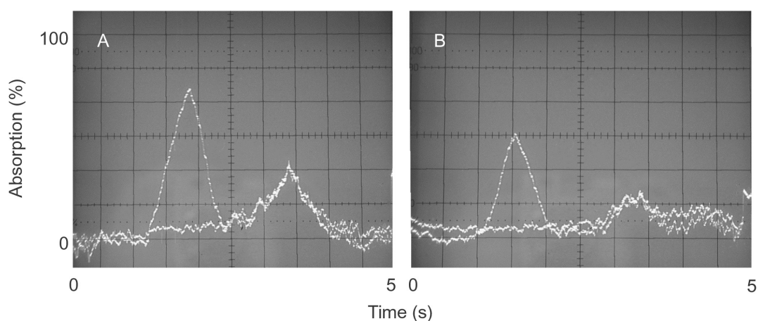
Figure 6. Absorption-time profiles of cadmium resulting from atomization of different biological samples employing the direct »tape sandwich« introduction technique; A – Mussel Tissue; B – Sea Lettuce.
