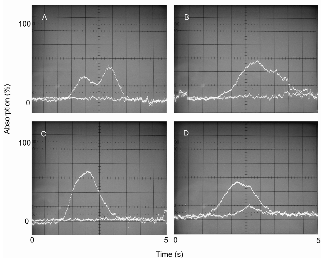
Figure 4. Absorption-time profiles of lead resulting from atomization of different plant materials employing the direct »tape sandwich« and slurry introduction techniques; A – lettuce – direct introduction: B – Sea Lettuce – direct introduction: C – lettuce – slurry introduction: D – Sea Lettuce – slurry introduction.
