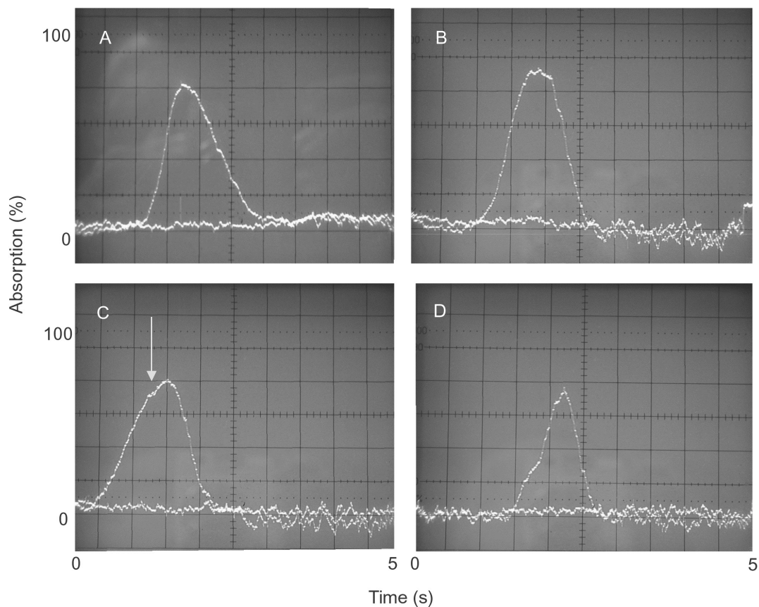
Figure 5. Absorption-time profiles of cadmium resulting from atomization of aqueous standard and various biological solid samples employing the direct »tape sandwich« introduction technique; A – CdCl 2 ; B – powdered hair; C – cabbage; D – bovine liver.
