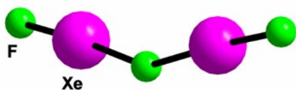
Figure 3. V-shaped cation \text{Xe}_2\text{F}_3^+ in the compounds \text{Xe}_2\text{F}_3\text{AF}_6 ( A = \text{As}, \text{Sb}, \text{Ru} )
