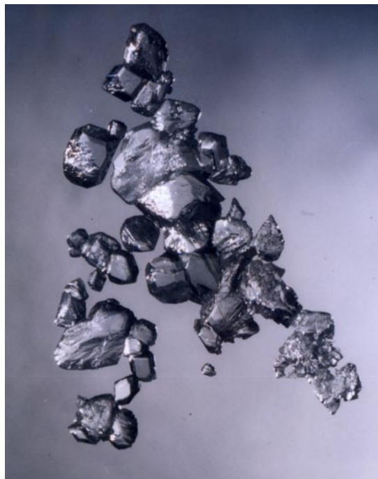
Figure 2. Crystals of XeF 2
