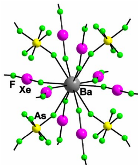
Figure 10. Example of the metal coordinated by bridging molecules of \text{XeF}_2 ; [\text{Ba}(\text{XeF}_2)_5](\text{AsF}_6)_2
