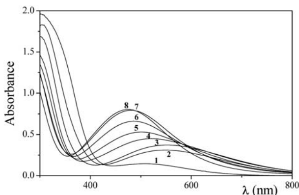
Fig. 4: Absorbance spectra of the iron(III) complex with hydroxyurea in dimethylformamide at various ligand concentrations. Conditions: c_{\text{Fe}} = 5 \times 10^{-4} M, c_{\text{HU}} = 0 (1), 2.5 \times 10^{-4} (2), 5 \times 10^{-4} (3), 2.5 \times 10^{-3} (4), 5 \times 10^{-3} (5), 1 \times 10^{-2} (6), 1.5 \times 10^{-2} (7) and 3 \times 10^{-2} M (8), T = 25 °C.
