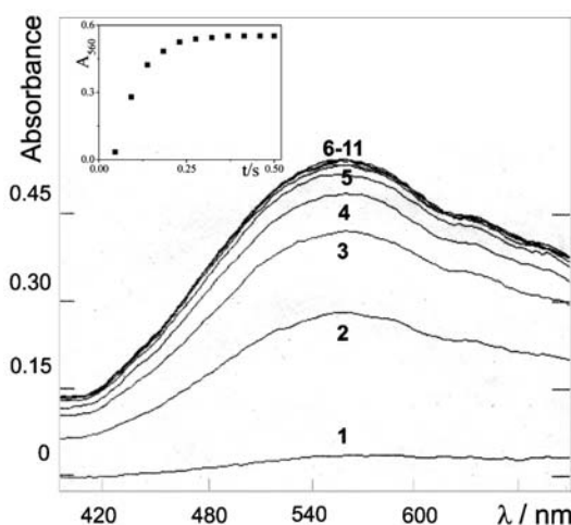
Fig. 1: Visible spectra recorded after mixing solution of hydroxyurea ( 1.15 \times 10^{-1} M) with iron(III) ( 1.15 \times 10^{-3} M). The last spectrum was taken after 0.5 seconds. Conditions: c_{\text{H}^+} = 4 \times 10^{-2} , I = 2.0 M ( \text{NaClO}_4 ), T = 25 °C. Inset: The absorbance at 560 nm versus time dependence for the same reaction.
