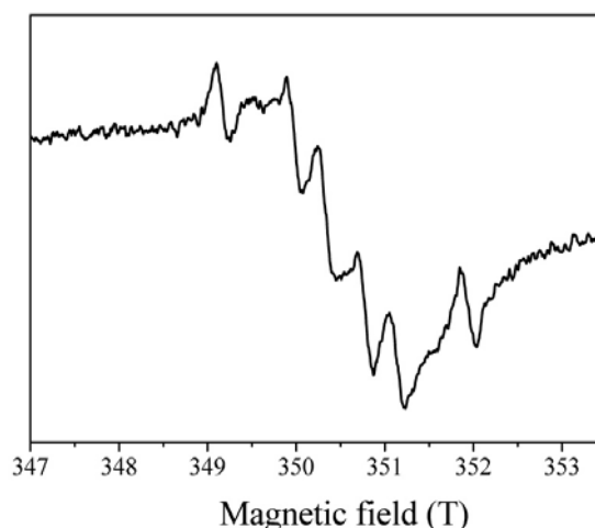
Fig. 6: EPR spectrum recorded under conditions of an excess of hydroxyurea over iron(III) in dimethylformamide solution at room temperature with microwave frequency 9.85 GHz and microwave power of 2 mW. Conditions: c_{\text{Fe}} = 1 \times 10^{-3} M, c_{\text{HU}} = 5 \times 10^{-2} M.
