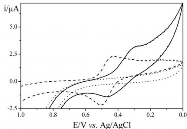
Fig. 5: Cyclic voltammograms of hydroxyurea (dotted line), its complex with iron(III) for c_L/c_{\text{Fe}} = 50:1 (solid line) and free iron(III) species (dashed line). Conditions: c_{\text{HU}} = 5 \times 10^{-2} M, dimethylformamide and 0.1 M \text{LiClO}_4 ; Pt working electrode at 100 \text{mVs}^{-1} scan rate, potential expressed with respect to Ag/AgCl.
