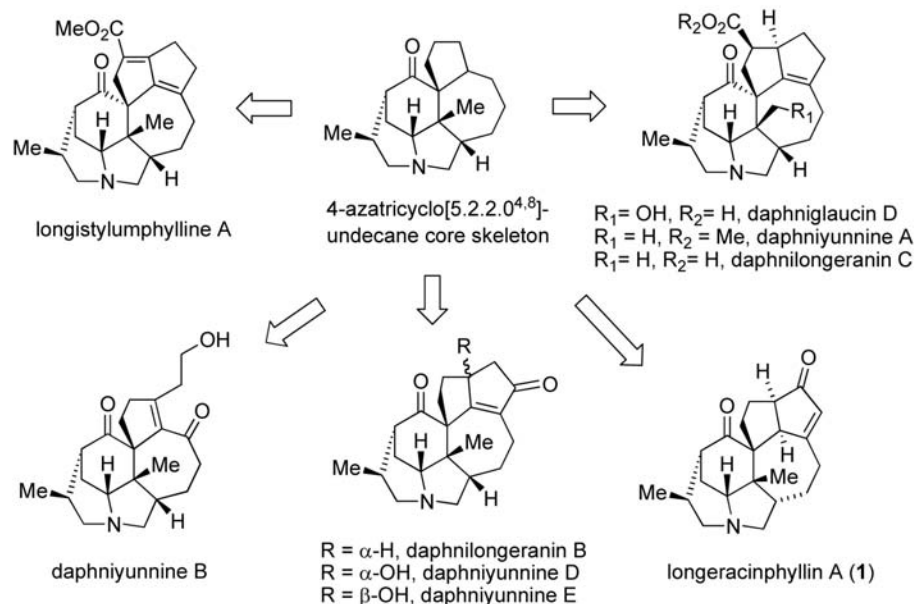
Figure 1. Structures of some Daphniphyllum Alkaloids
