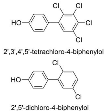
Figure 7. Structures of 4-OH-PCBs.
