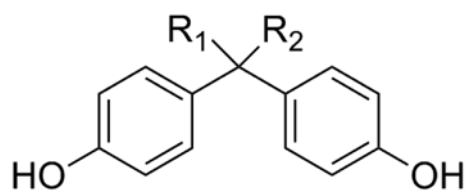
Bisphenol A ( R_1=CH_3 and R_2=CH_3 ) Bisphenol F ( R_1=H and R_2=H ) Bisphenol AF ( R_1=CF_3 and R_2=CF_3 ) Bisphenol B ( R_1=CH_3 and R_2=CH_3CH_2 )
