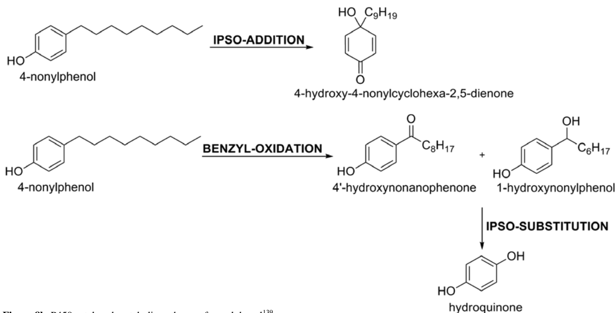
Figure 8b. P450 catalysed metabolic pathway of nonylphenol 139
