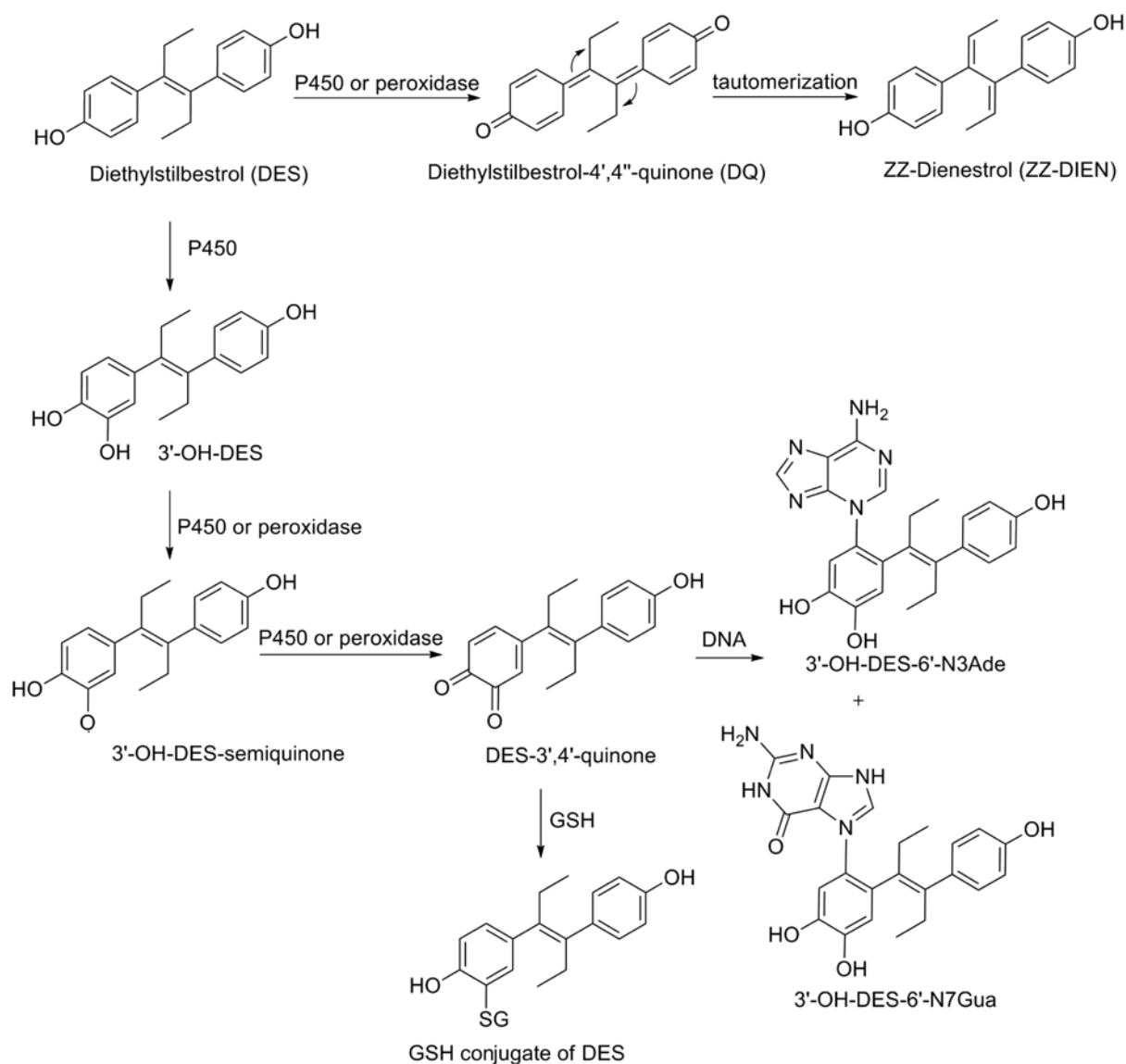
Figure 4. In vitro and in vivo metabolism of DES by cytochrome P450 or peroxidase 110,114
