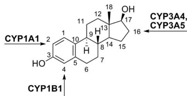
Figure 2. The most common P450s that take part in C-2, C-4 and C-16 hydroxylations of E2 in vitro 96-98
