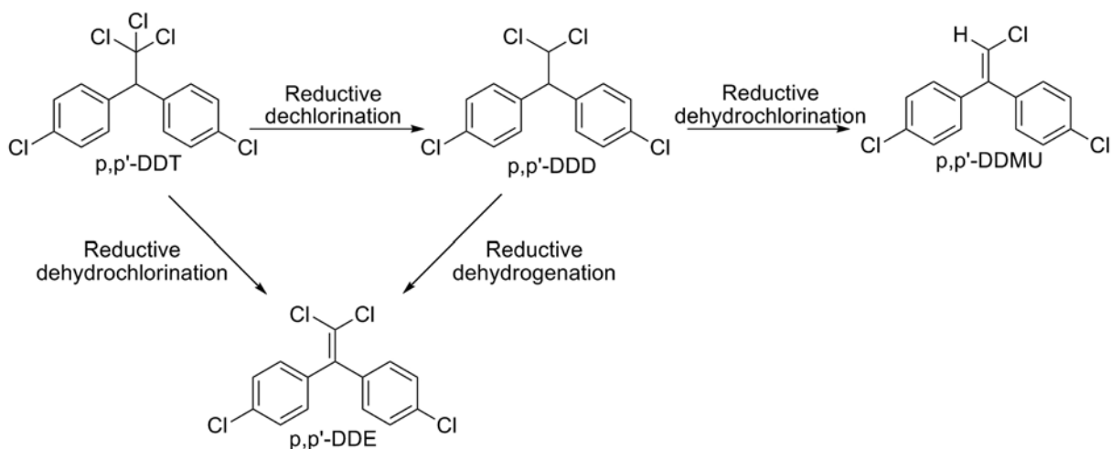
Figure 6a. Reductive metabolism of p,p'-DDT in rat liver microsomes by Kitamura et al. 127
