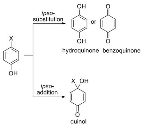
Figure 8a. P450 catalysed ipso -position reaction of para-substituted phenols 139
