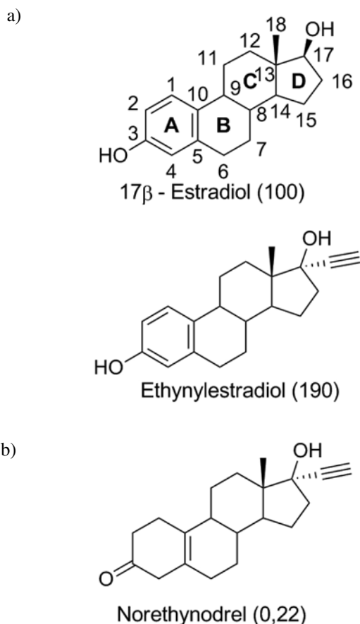
Figure 1. Steroids (a) with and (b) without phenolic structure (ring A); In each case the ratio of its binding affinity to that of E2 is expressed as a percentage given in parentheses. 2
