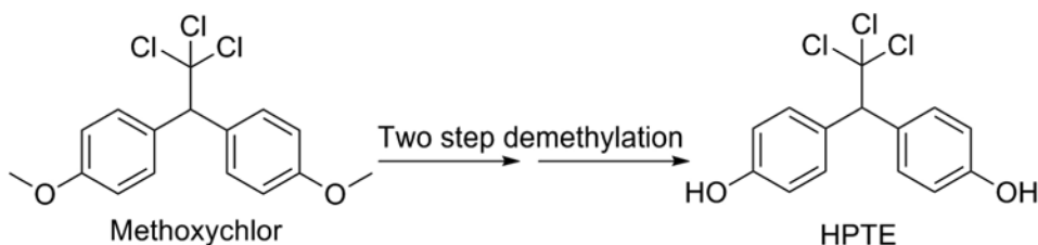
Figure 6b. Kupfer et al. proposed a two step demethylation of methoxychlor by using liver microsomes. 130
