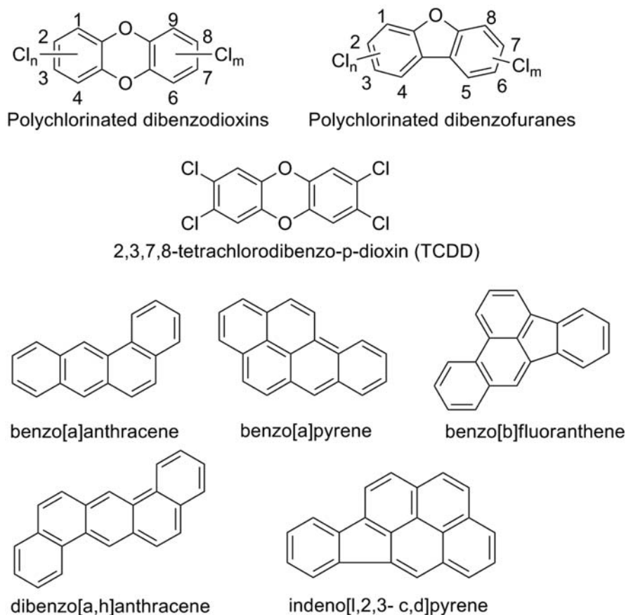
Figure 9. Structures of PCDDs, PCDFs and five PAHs that are known human carcinogens
