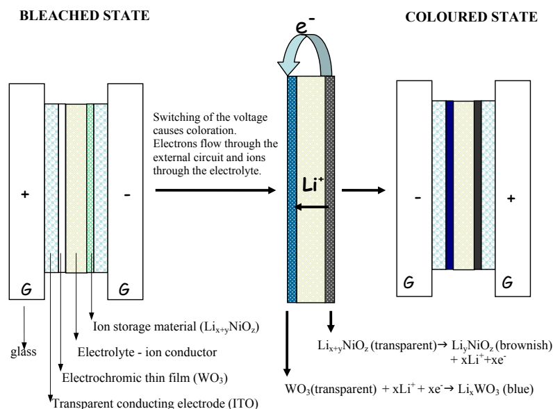
Figure 1. Construction of a basic ECD ( \text{WO}_3/\text{electrolyte}/\text{Li}_{x+y}\text{NiO}_2 ) and reactions on coloration.
